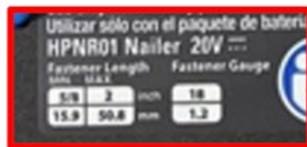
Hart 18-Gauge 2” Brad Nailer with location of Model Number
